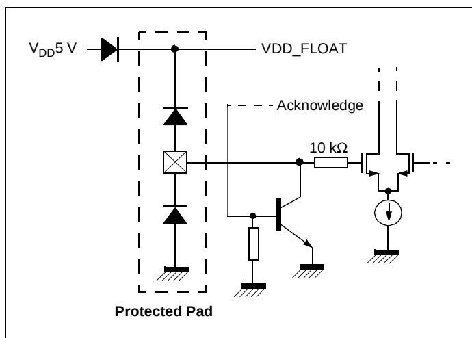
Figure 16: I 2 C Bus SDA I/O (Pin 38)
